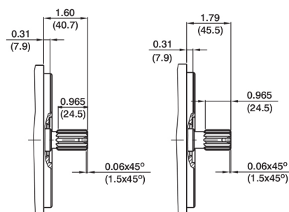
Shaft code 4 SAE BB splined shaft Class 1-J498b 16/32 dp. 15 teeth 30° pressure angle flat root side fit
